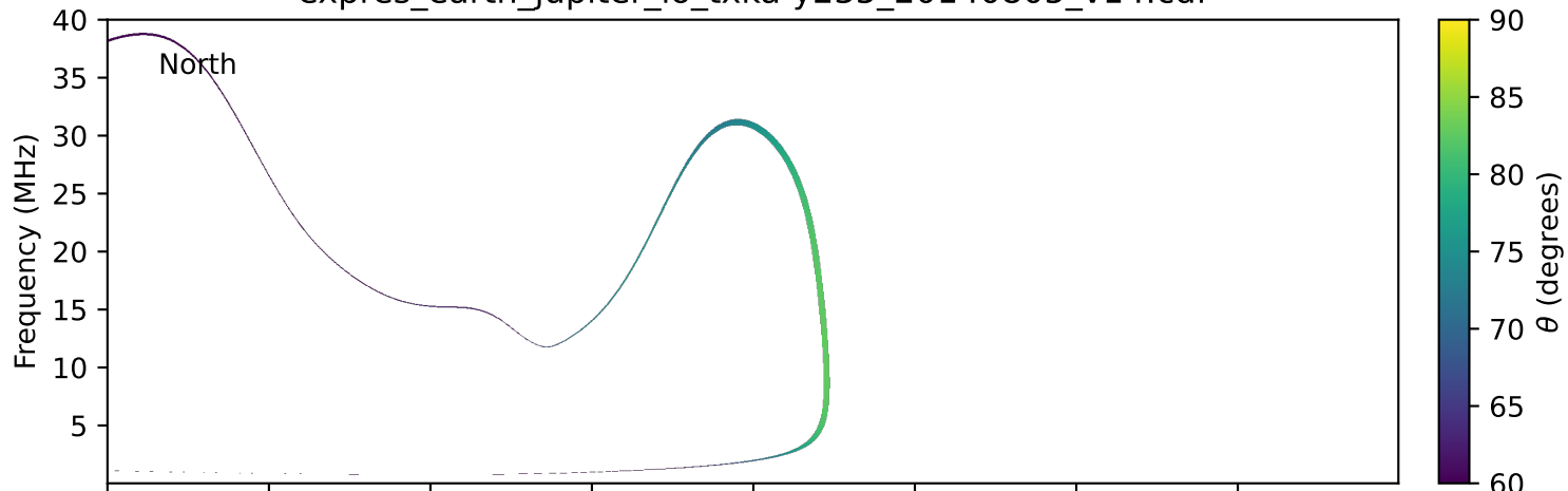
expres_earth_jupiter_io_txka-y235_20140805_v14.cdf
