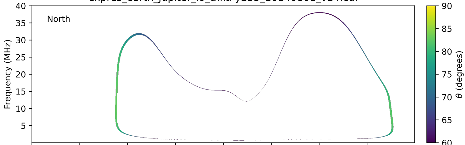
expres_earth_jupiter_io_txka-y235_20140801_v14.cdf
