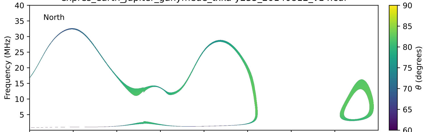
expres_earth_jupiter_ganymede_txka-y235_20140812_v14.cdf
