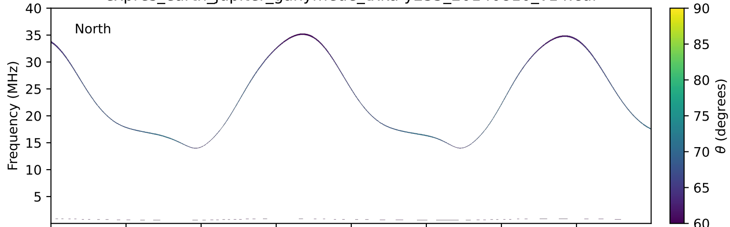
expres_earth_jupiter_ganymede_txka-y235_20140810_v14.cdf
