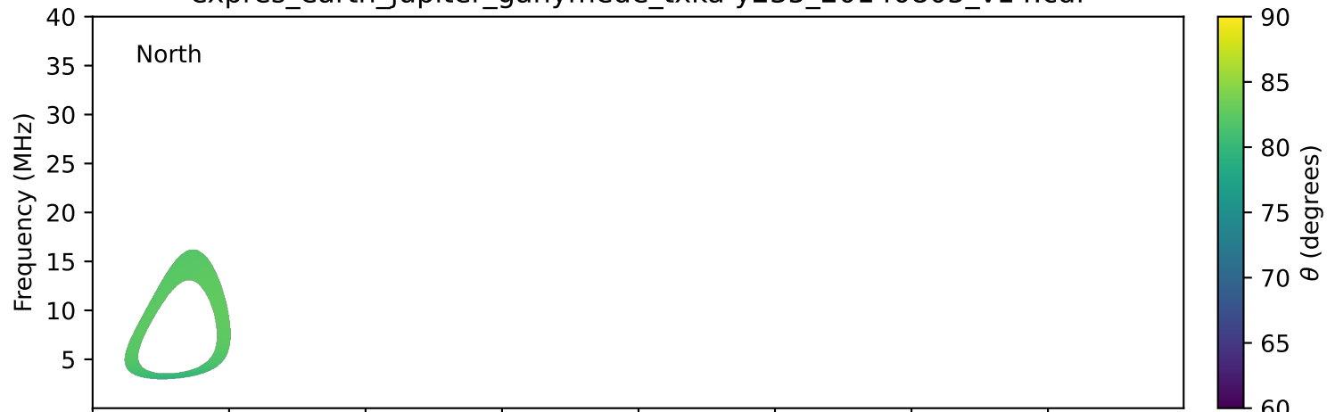
expres_earth_jupiter_ganymede_txka-y235_20140805_v14.cdf
