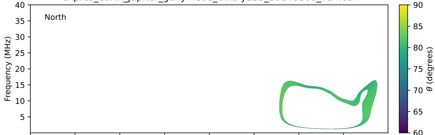
expres_earth_jupiter_ganymede_txka-y235_20140801_v14.cdf
