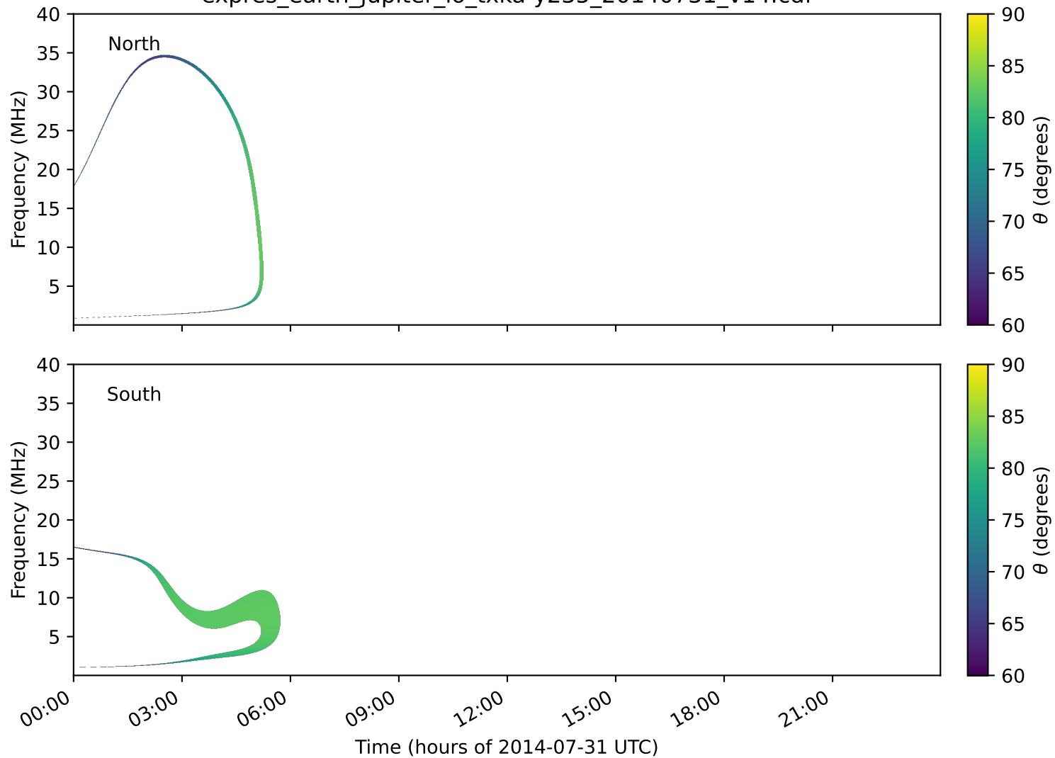
expres_earth_jupiter_io_txka-y235_20140731_v14.cdf
