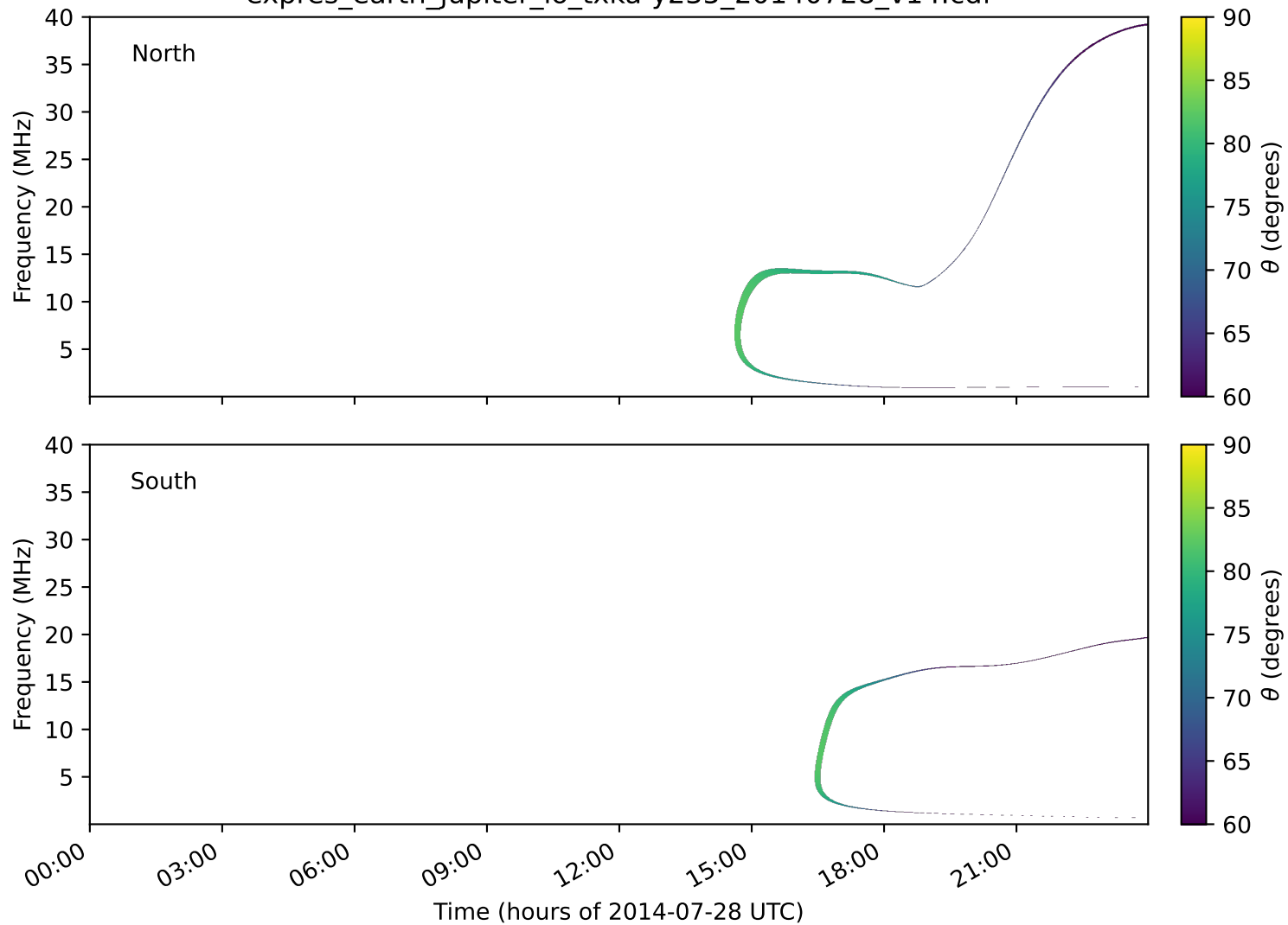
expres_earth_jupiter_io_txka-y235_20140728_v14.cdf
