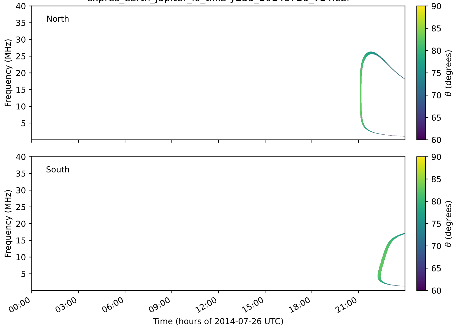
expres_earth_jupiter_io_txka-y235_20140726_v14.cdf
