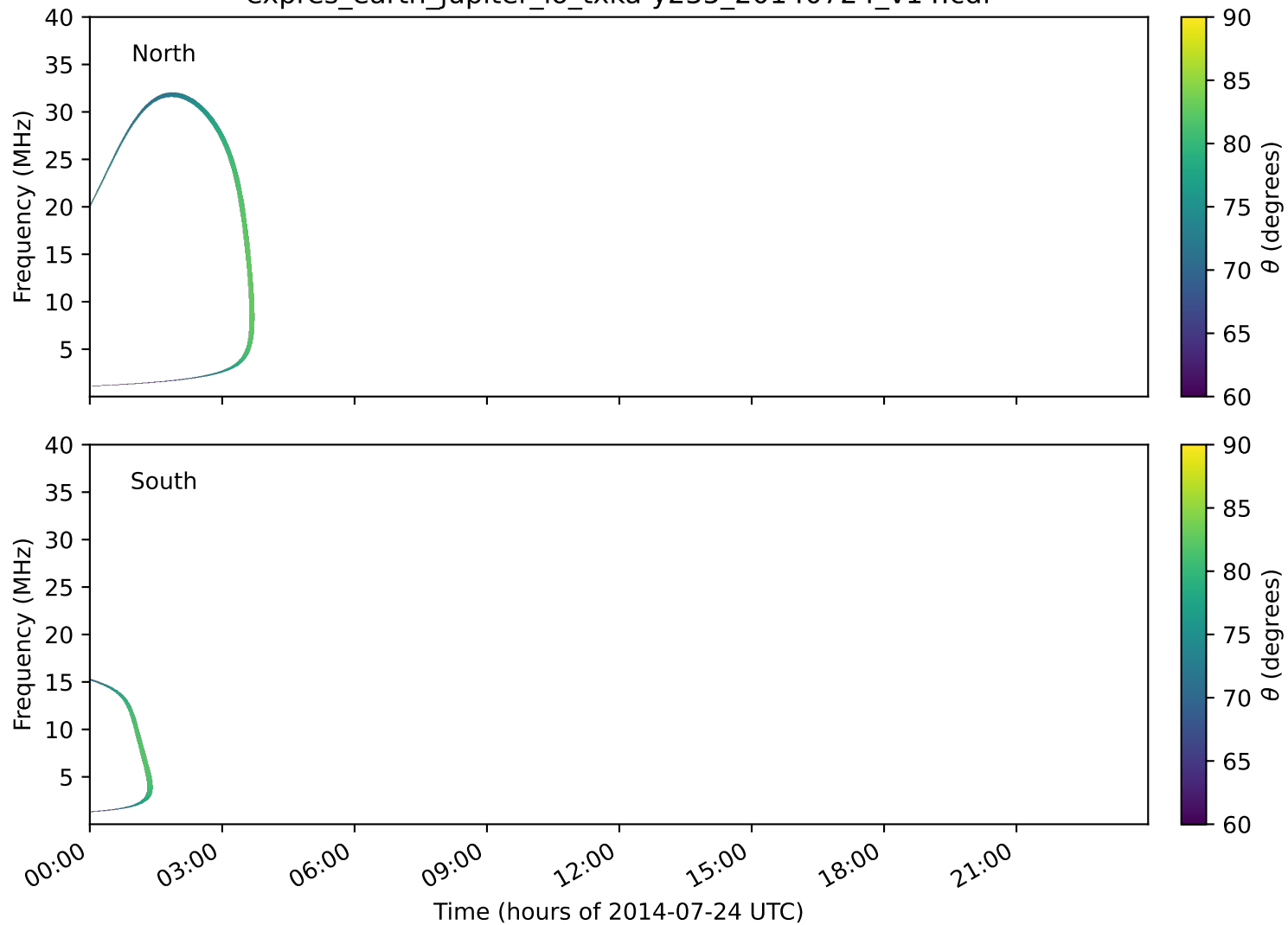
expres_earth_jupiter_io_txka-y235_20140724_v14.cdf
