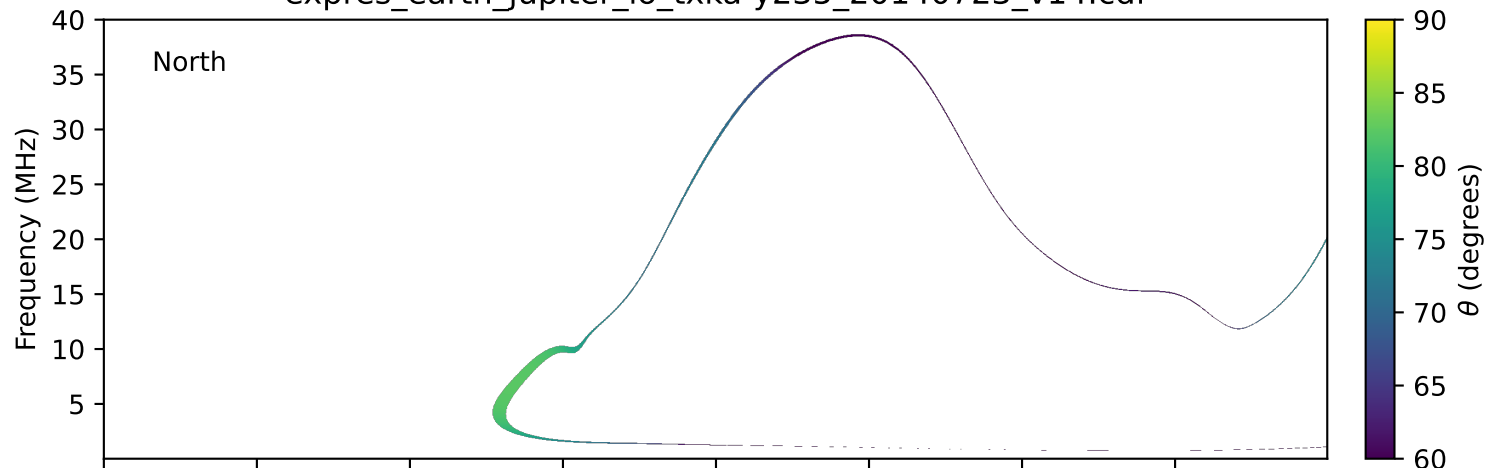
expres_earth_jupiter_io_txka-y235_20140723_v14.cdf
