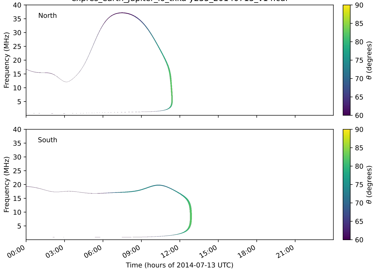
expres_earth_jupiter_io_txka-y235_20140713_v14.cdf
