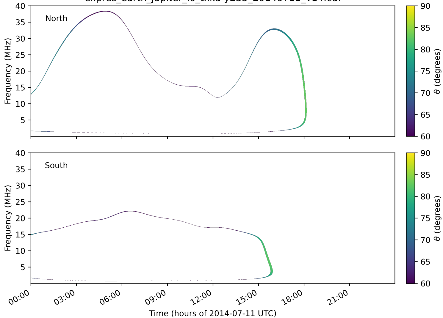
expres_earth_jupiter_io_txka-y235_20140711_v14.cdf
