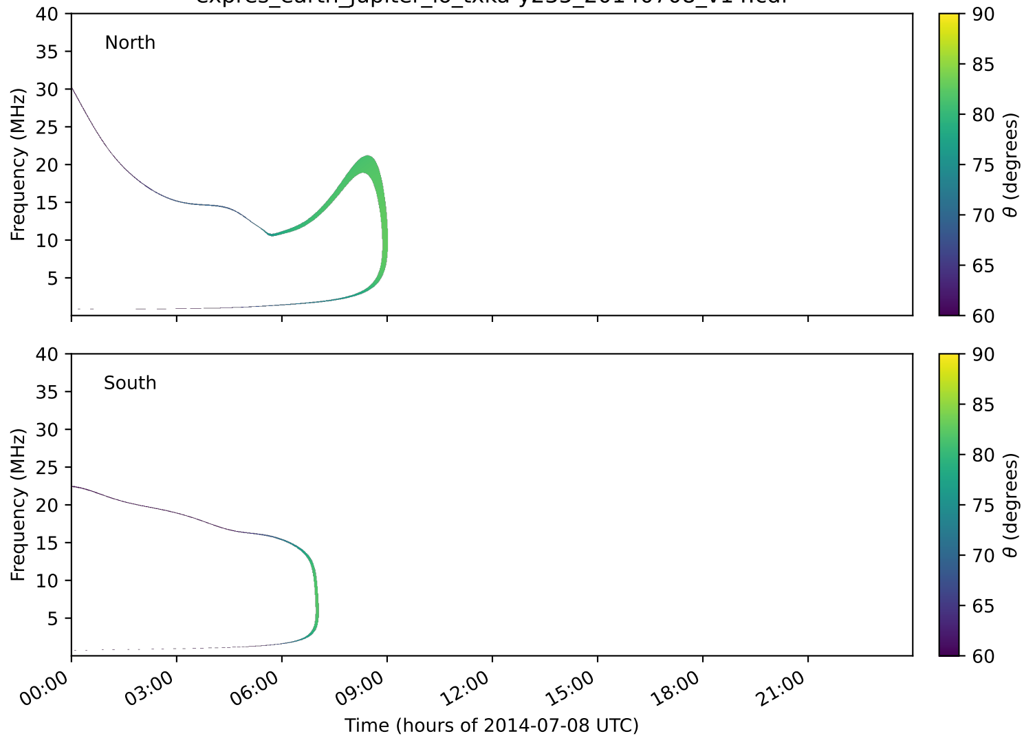
expres_earth_jupiter_io_txka-y235_20140708_v14.cdf
