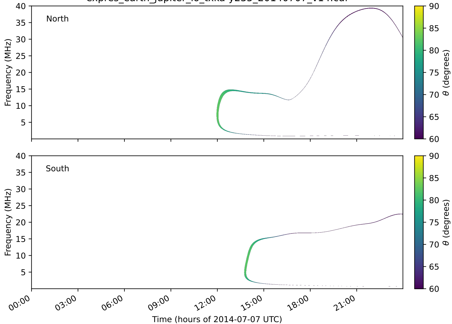
expres_earth_jupiter_io_txka-y235_20140707_v14.cdf
