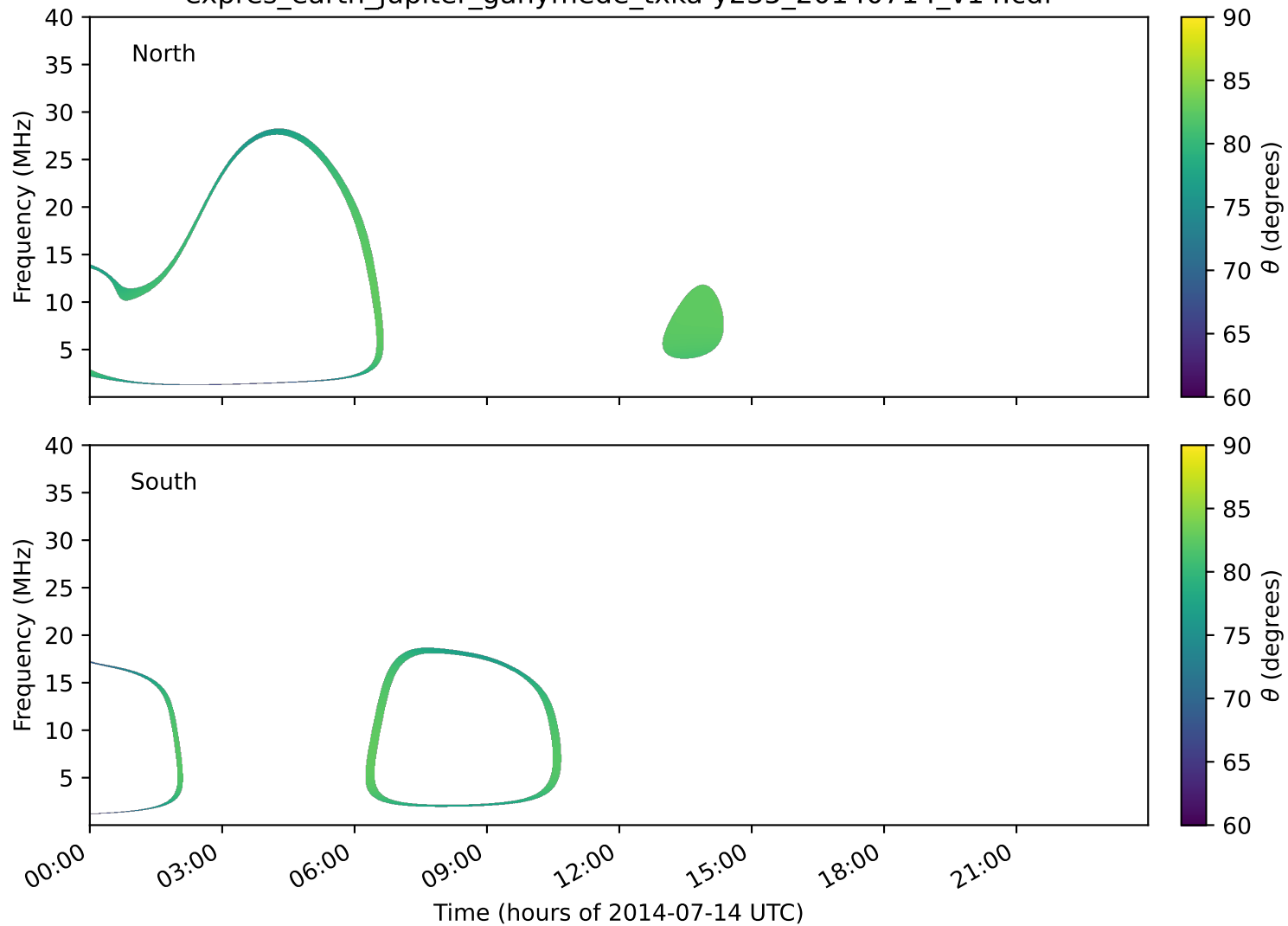
expres_earth_jupiter_ganymede_txka-y235_20140714_v14.cdf
