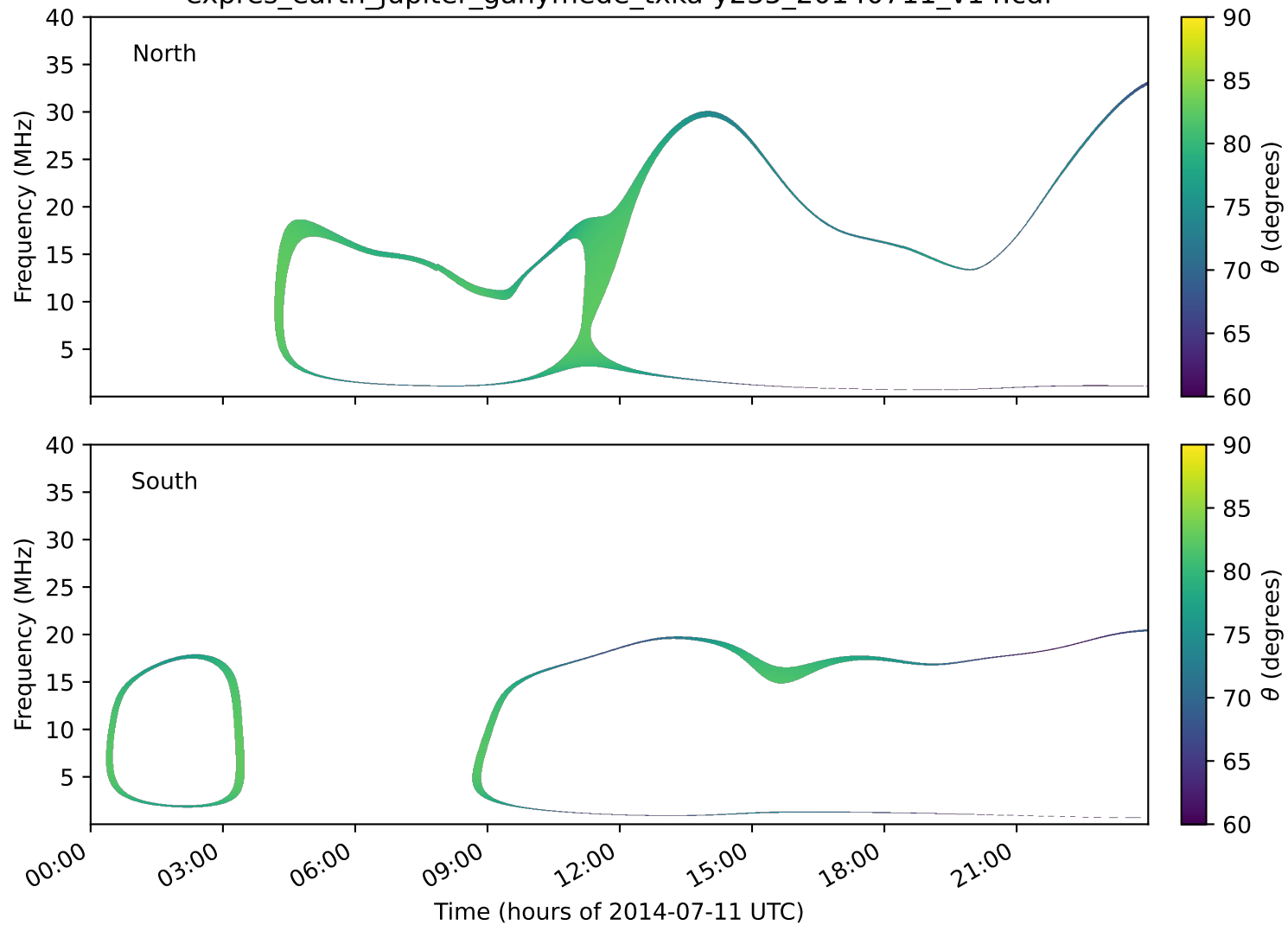
expres_earth_jupiter_ganymede_txka-y235_20140711_v14.cdf
