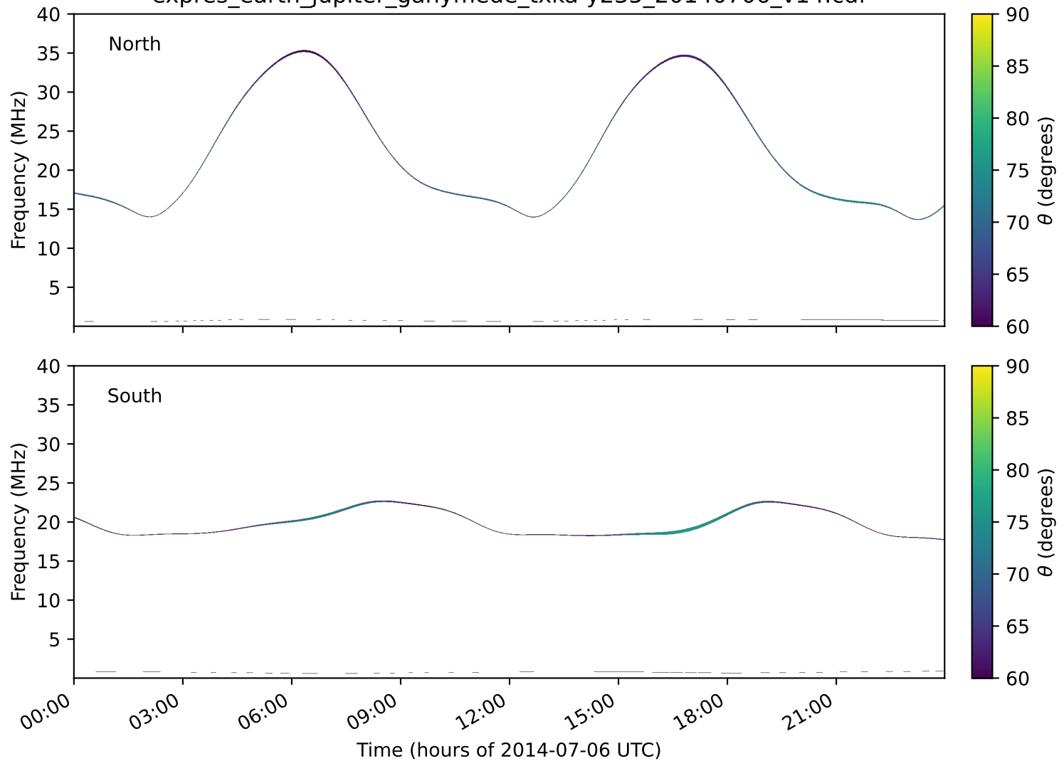
expres_earth_jupiter_ganymede_txka-y235_20140706_v14.cdf
