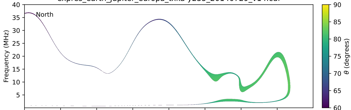
expres_earth_jupiter_europa_txka-y235_20140729_v14.cdf
