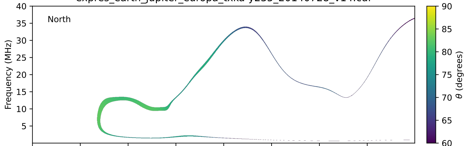
expres_earth_jupiter_europa_txka-y235_20140728_v14.cdf
