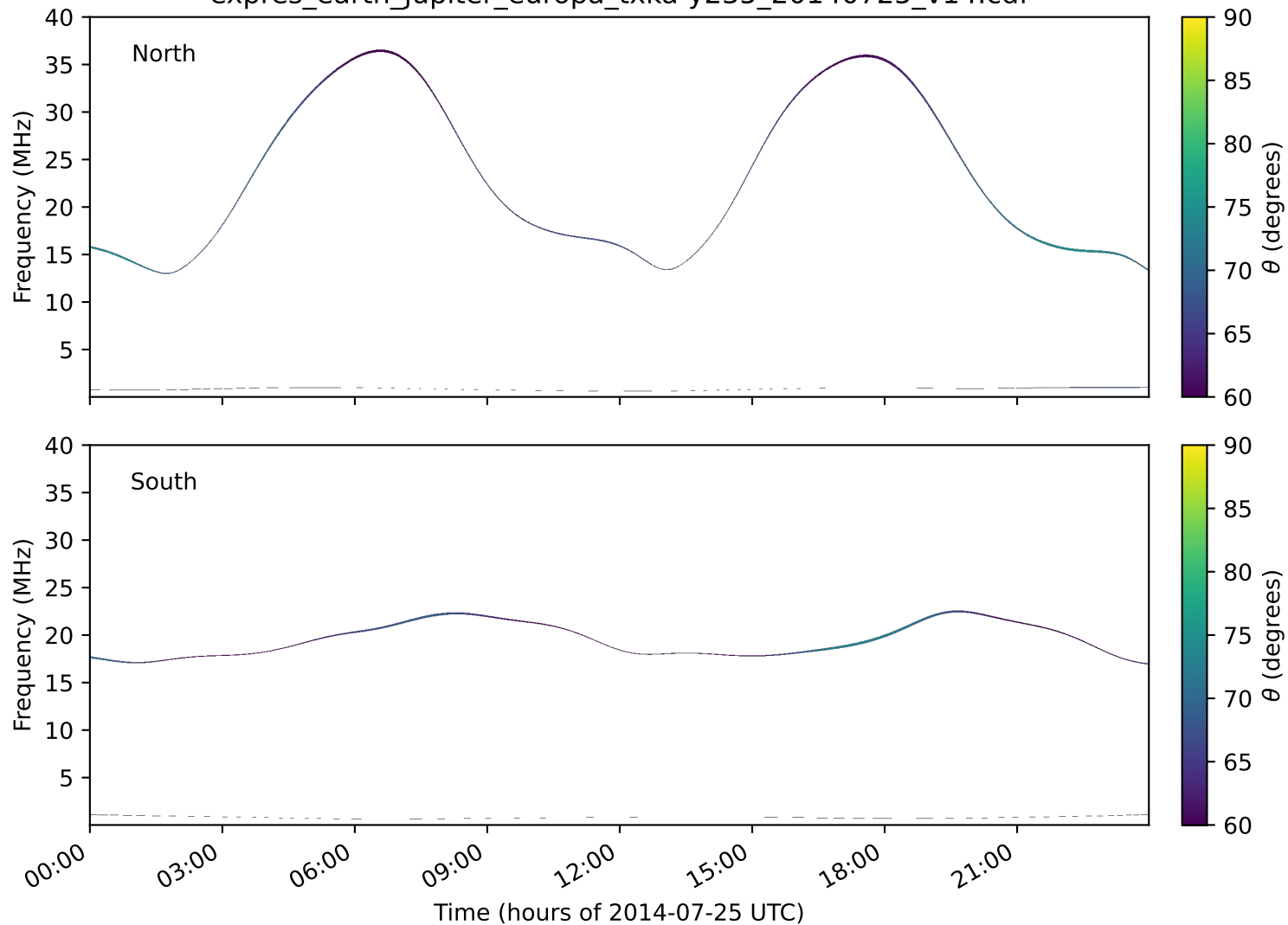
expres_earth_jupiter_europa_txka-y235_20140725_v14.cdf
