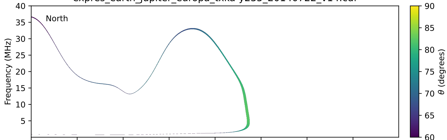
expres_earth_jupiter_europa_txka-y235_20140722_v14.cdf
