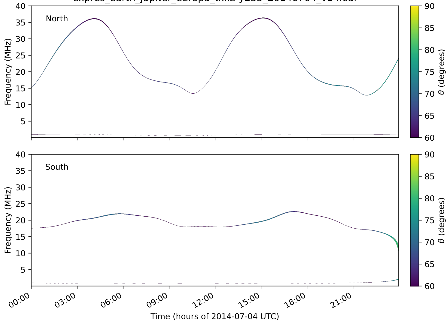
expres_earth_jupiter_europa_txka-y235_20140704_v14.cdf
