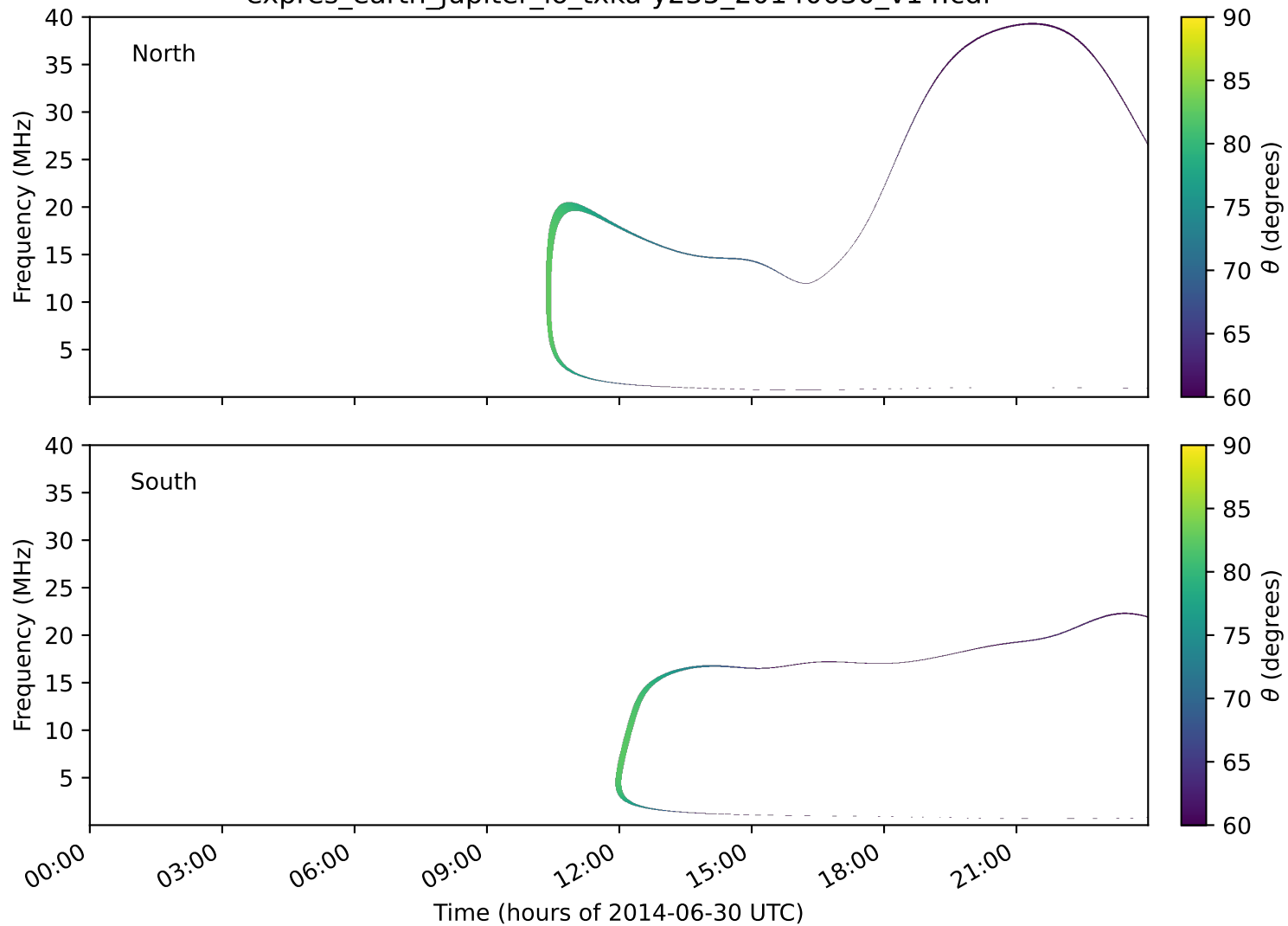
expres_earth_jupiter_io_txka-y235_20140630_v14.cdf
