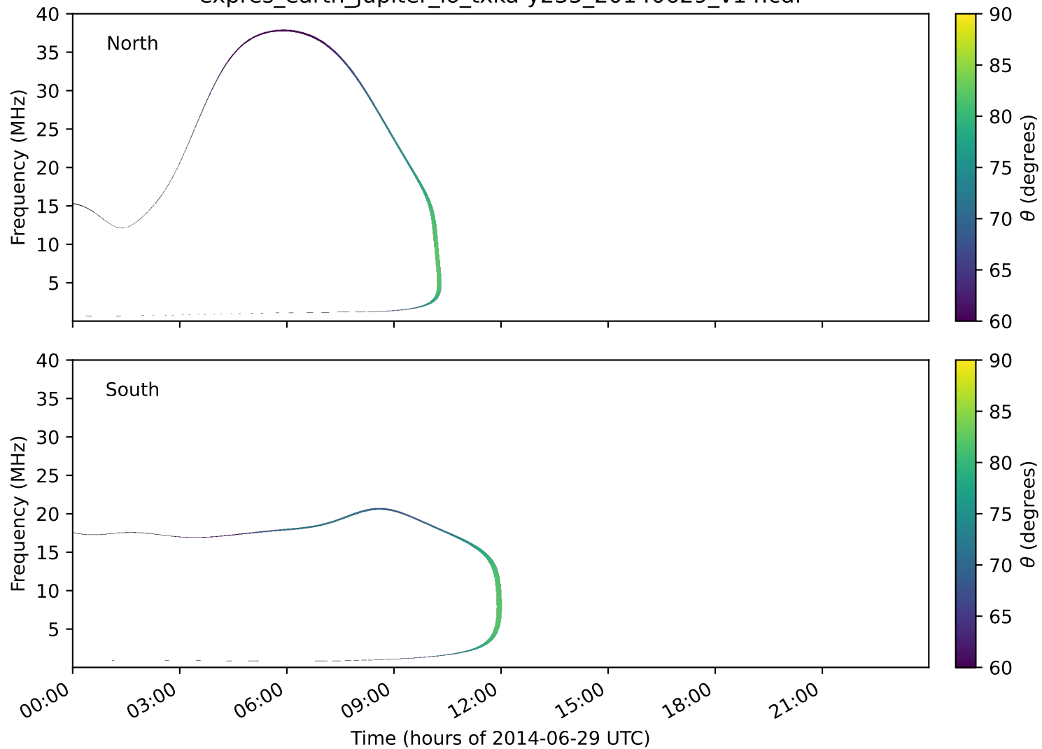
expres_earth_jupiter_io_txka-y235_20140629_v14.cdf
