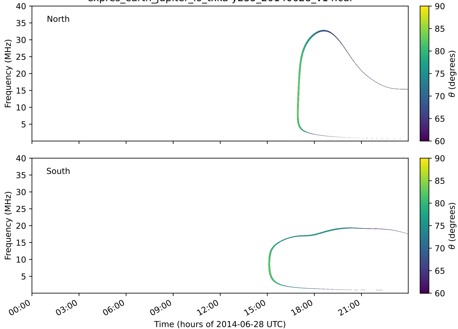
expres_earth_jupiter_io_txka-y235_20140628_v14.cdf
