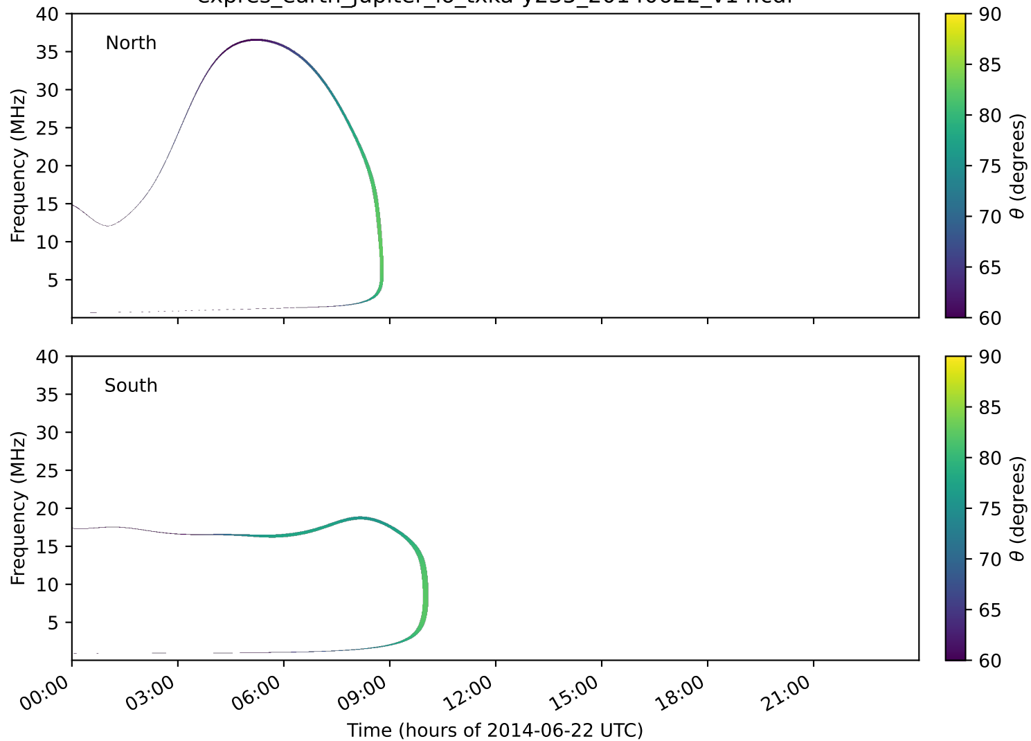
expres_earth_jupiter_io_txka-y235_20140622_v14.cdf
