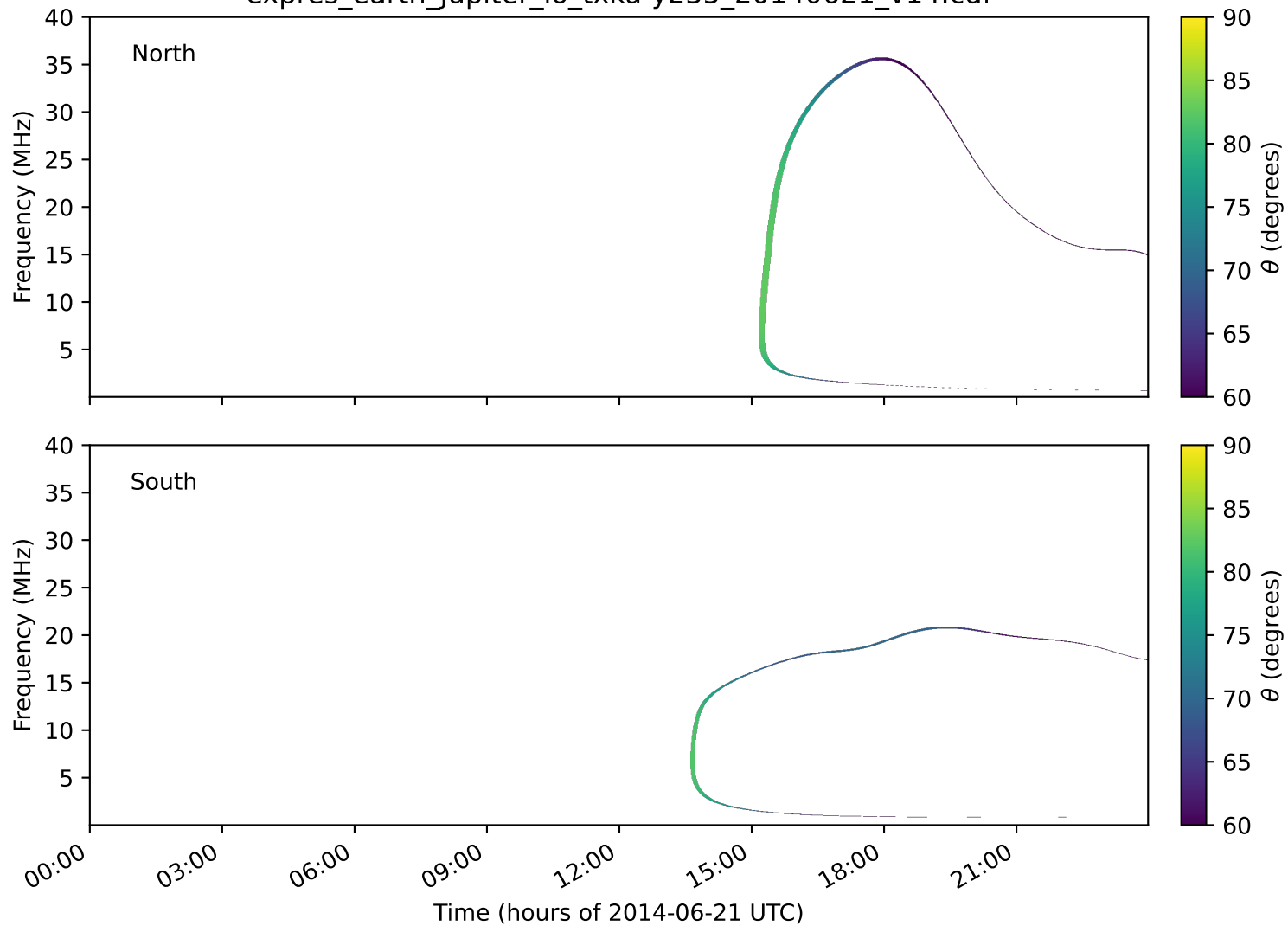
expres_earth_jupiter_io_txka-y235_20140621_v14.cdf
