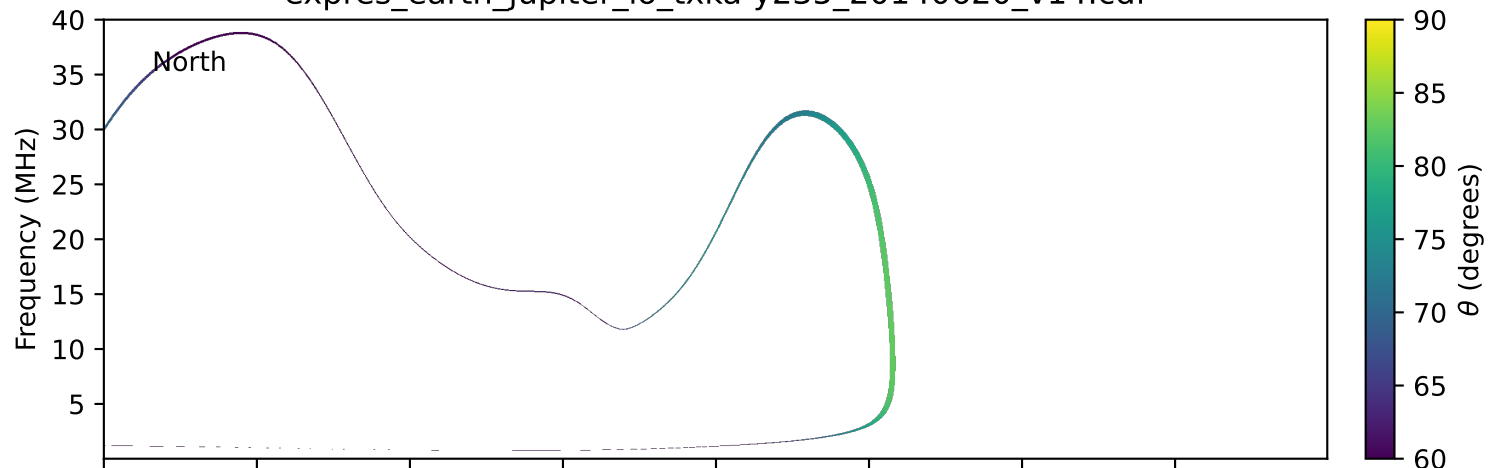
expres_earth_jupiter_io_txka-y235_20140620_v14.cdf
