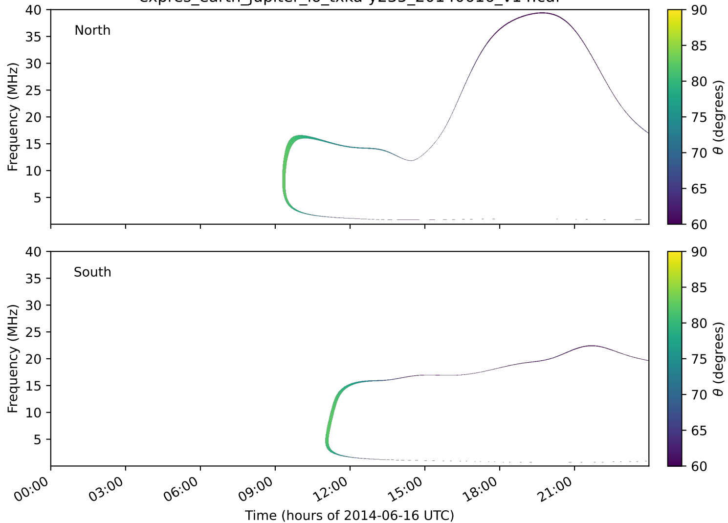
expres_earth_jupiter_io_txka-y235_20140616_v14.cdf
