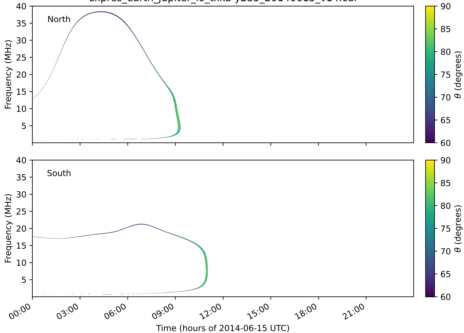
expres_earth_jupiter_io_txka-y235_20140615_v14.cdf
