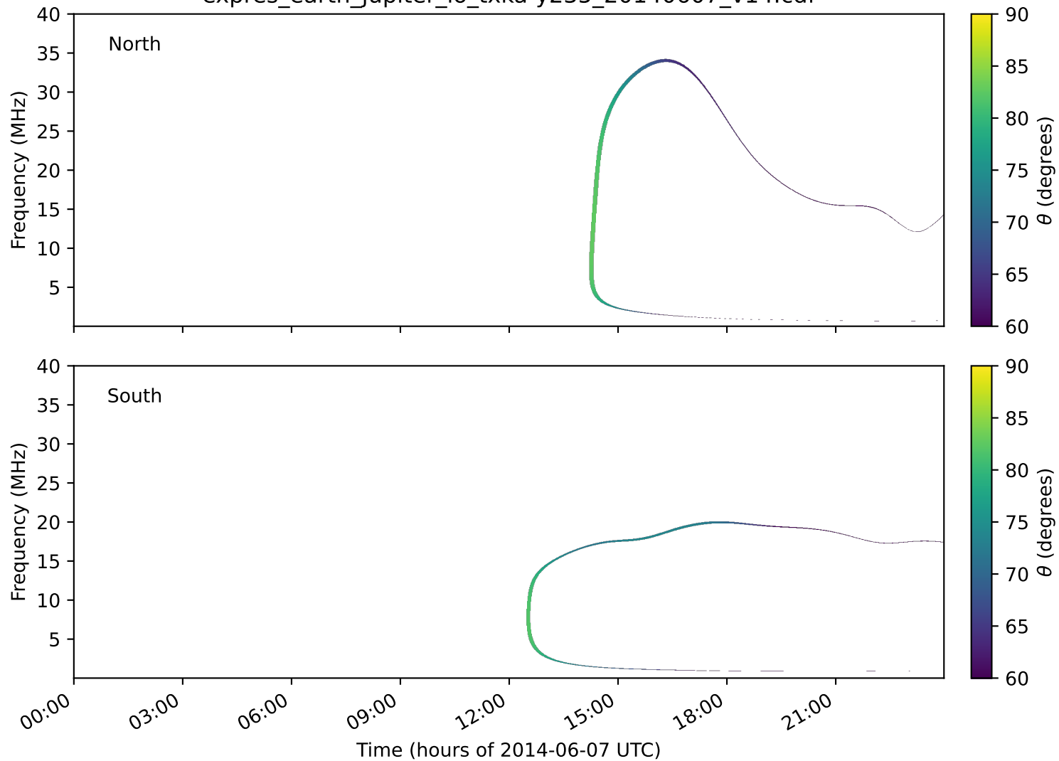
expres_earth_jupiter_io_txka-y235_20140607_v14.cdf
