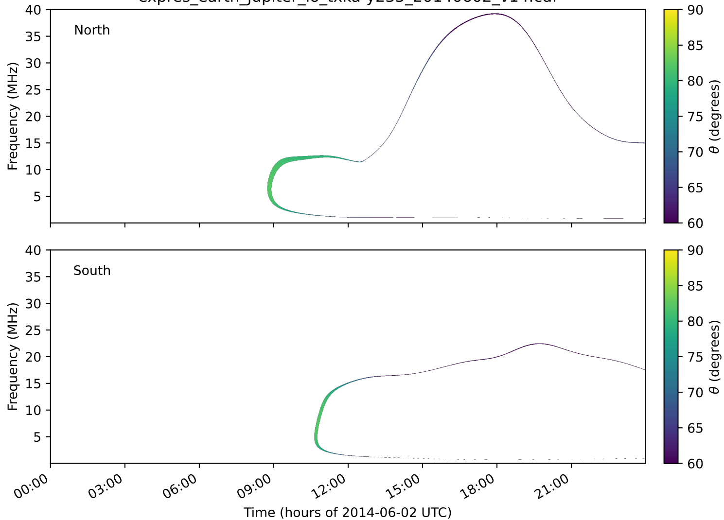
expres_earth_jupiter_io_txka-y235_20140602_v14.cdf
