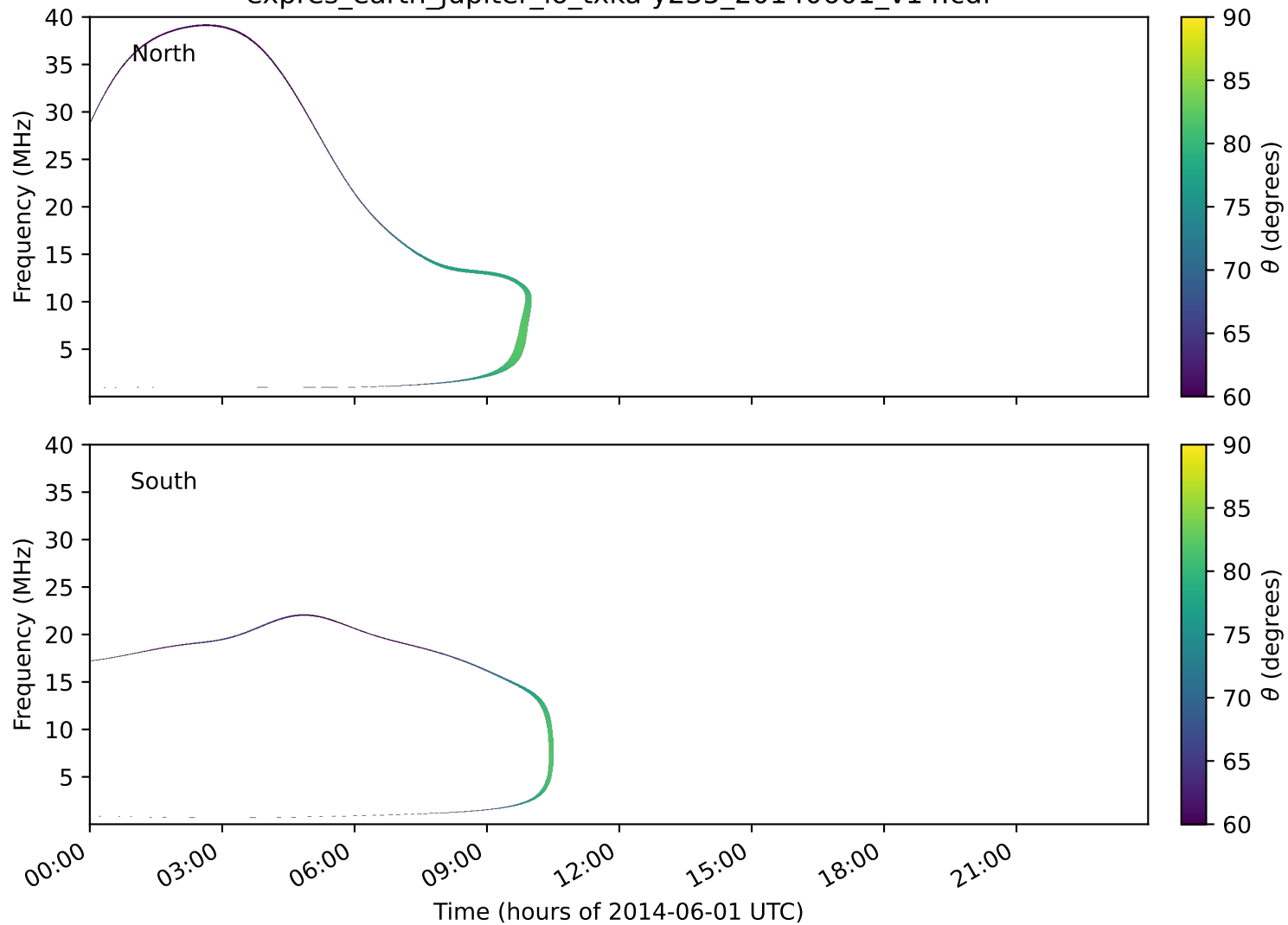
expres_earth_jupiter_io_txka-y235_20140601_v14.cdf
