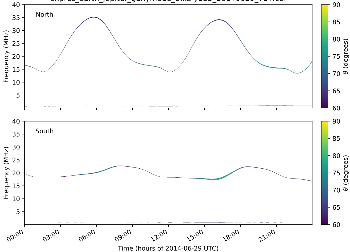
expres_earth_jupiter_ganymede_txka-y235_20140629_v14.cdf
