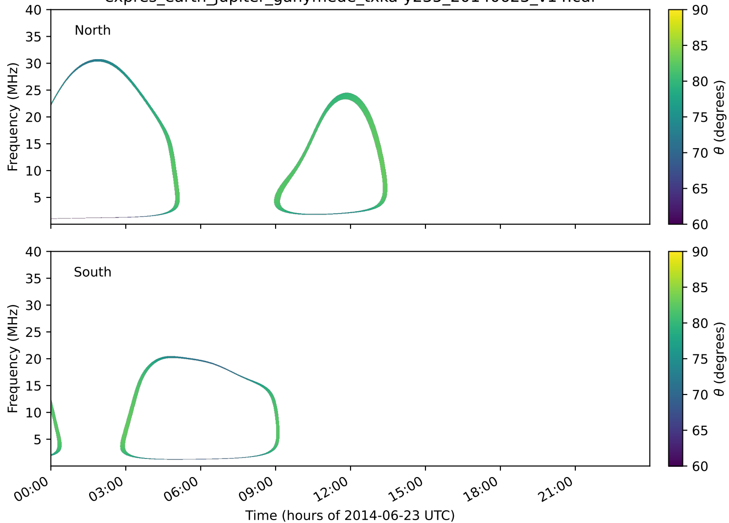
expres_earth_jupiter_ganymede_txka-y235_20140623_v14.cdf
