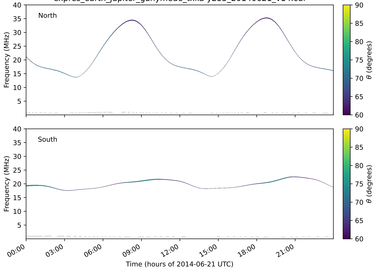
expres_earth_jupiter_ganymede_txka-y235_20140621_v14.cdf
