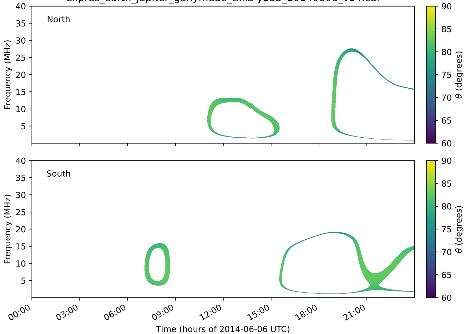
expres_earth_jupiter_ganymede_txka-y235_20140606_v14.cdf
