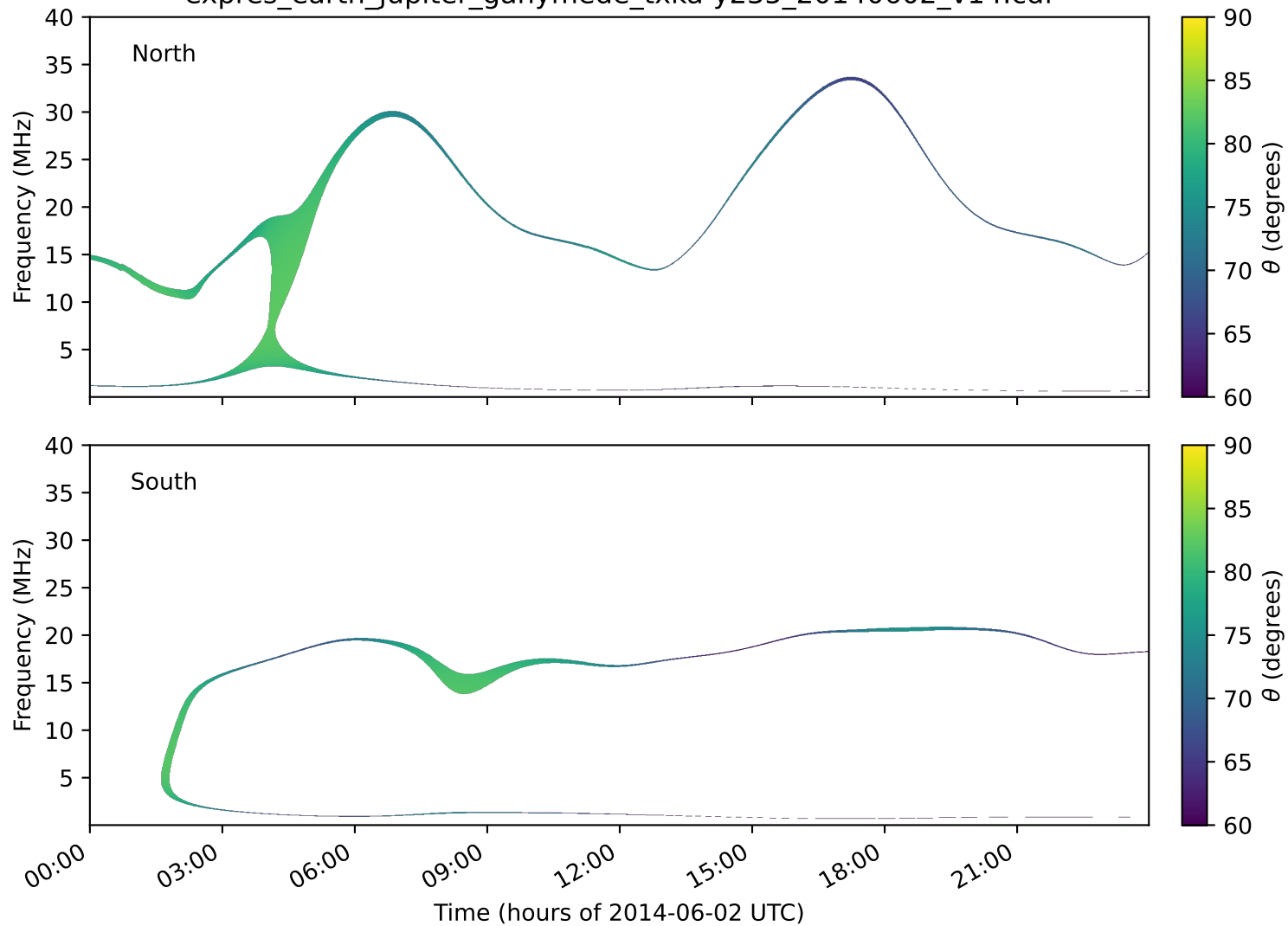
expres_earth_jupiter_ganymede_txka-y235_20140602_v14.cdf
