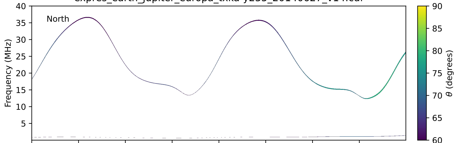
expres_earth_jupiter_europa_txka-y235_20140627_v14.cdf
