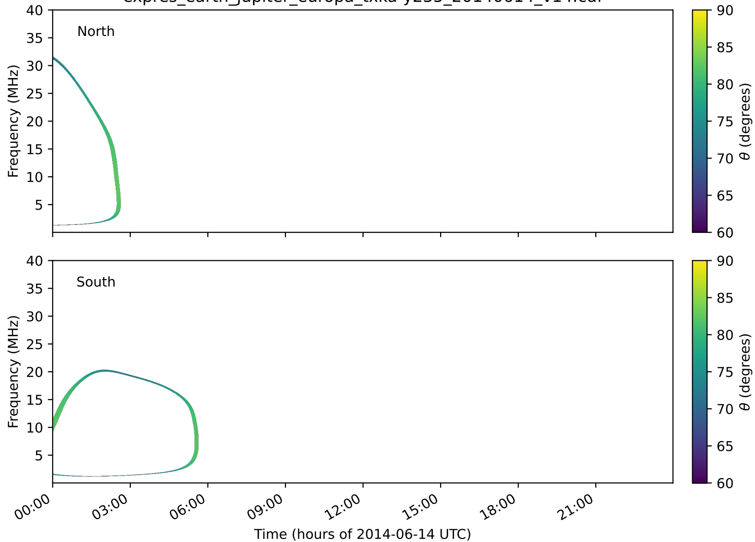
expres_earth_jupiter_europa_txka-y235_20140614_v14.cdf
