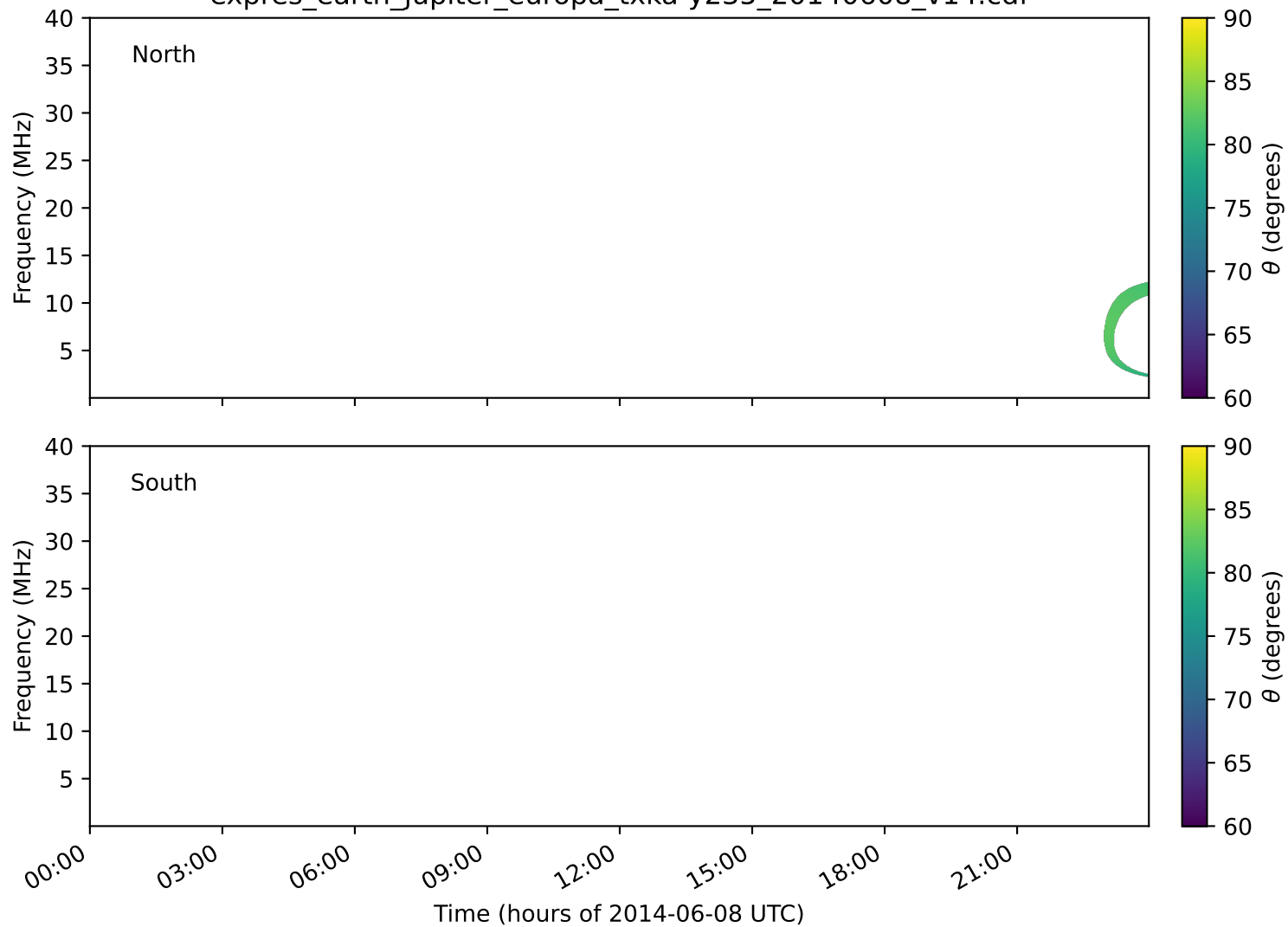
expres_earth_jupiter_europa_txka-y235_20140608_v14.cdf
