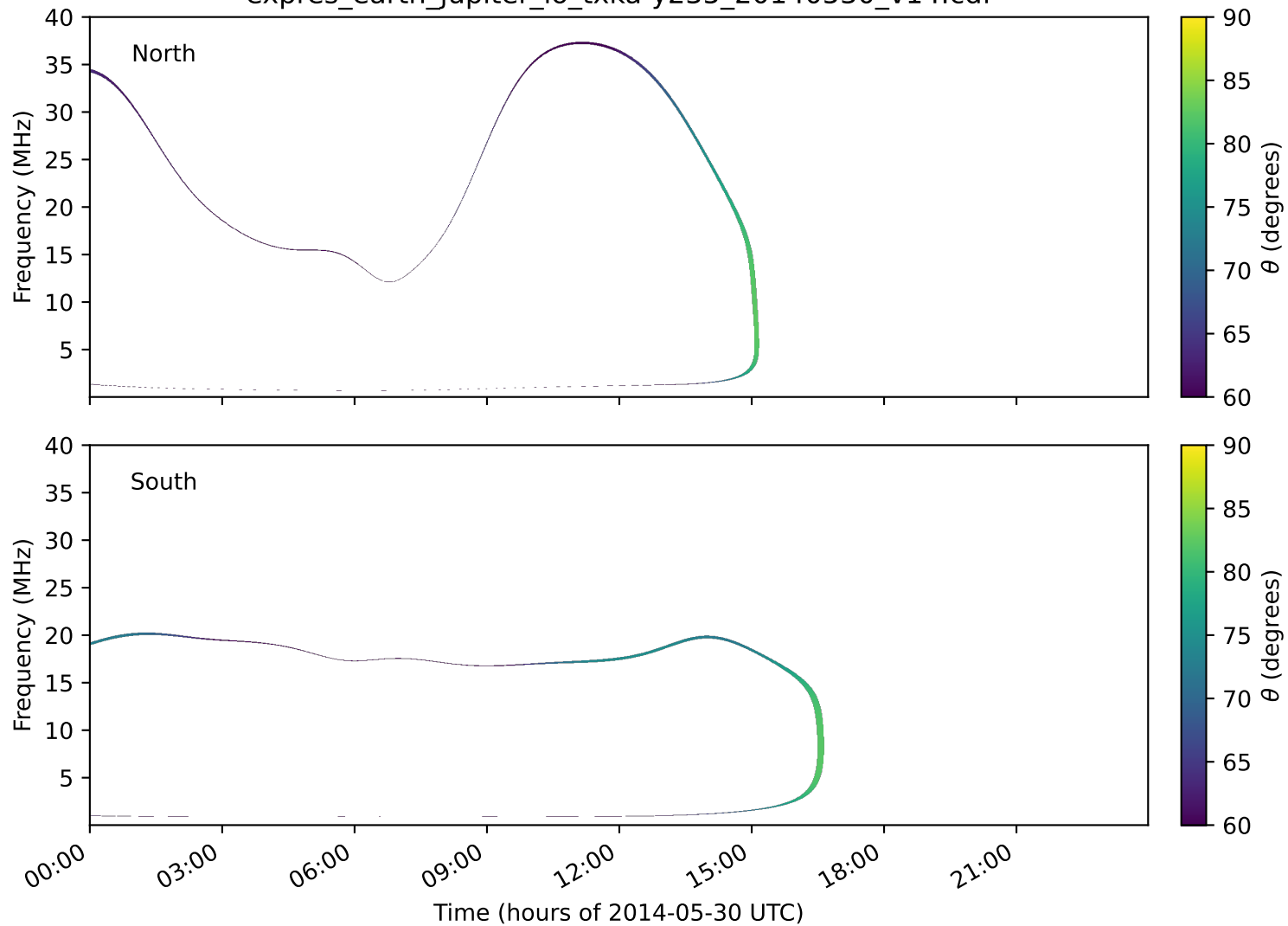
expres_earth_jupiter_io_txka-y235_20140530_v14.cdf
