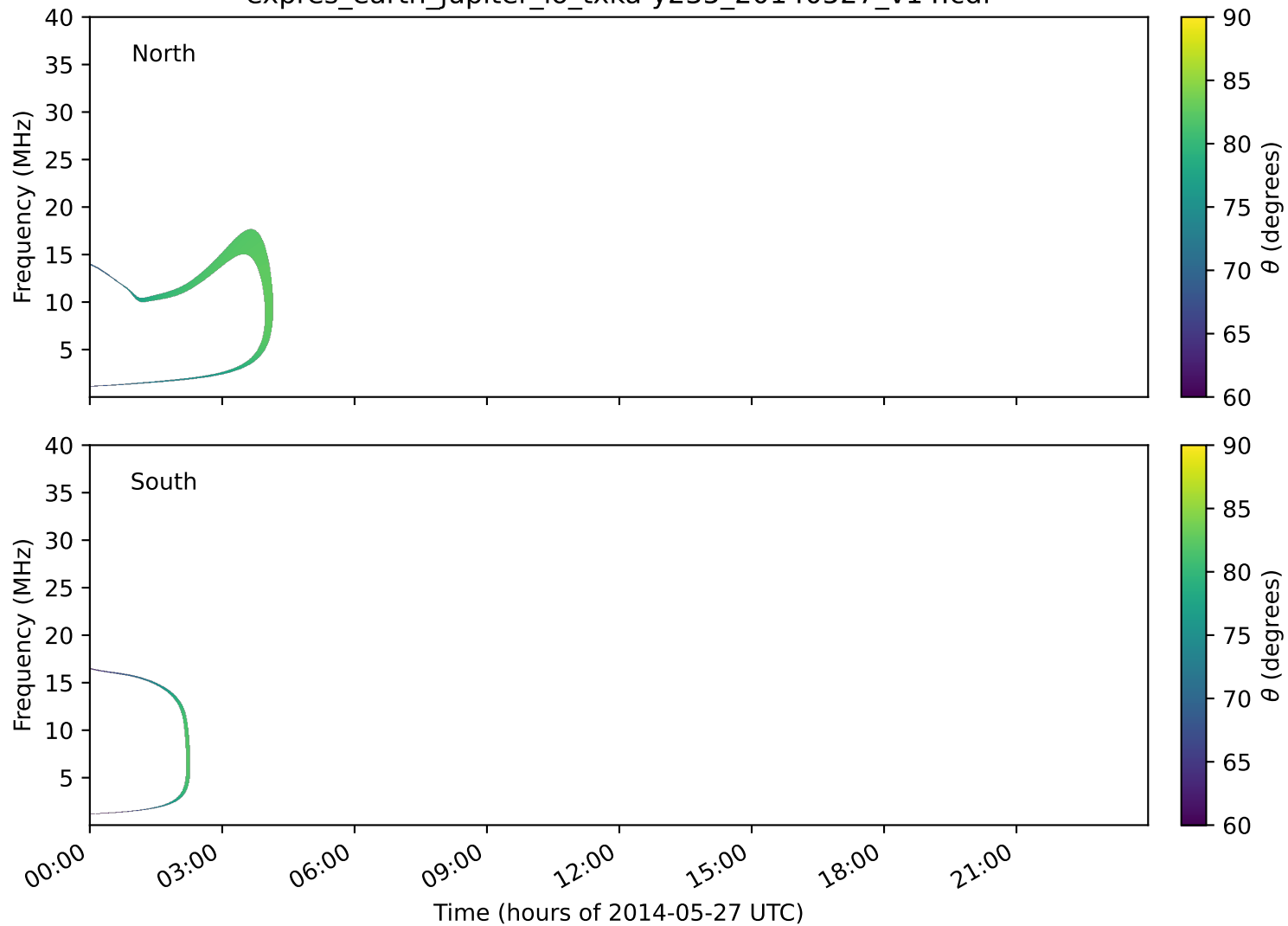
expres_earth_jupiter_io_txka-y235_20140527_v14.cdf
