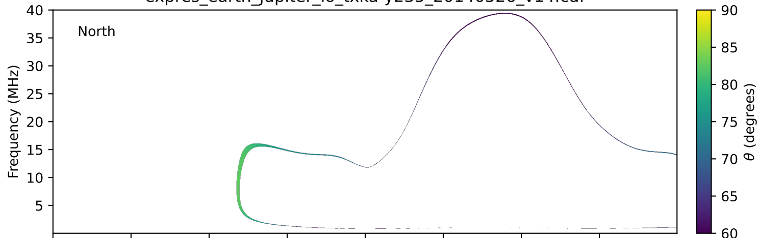
expres_earth_jupiter_io_txka-y235_20140526_v14.cdf
