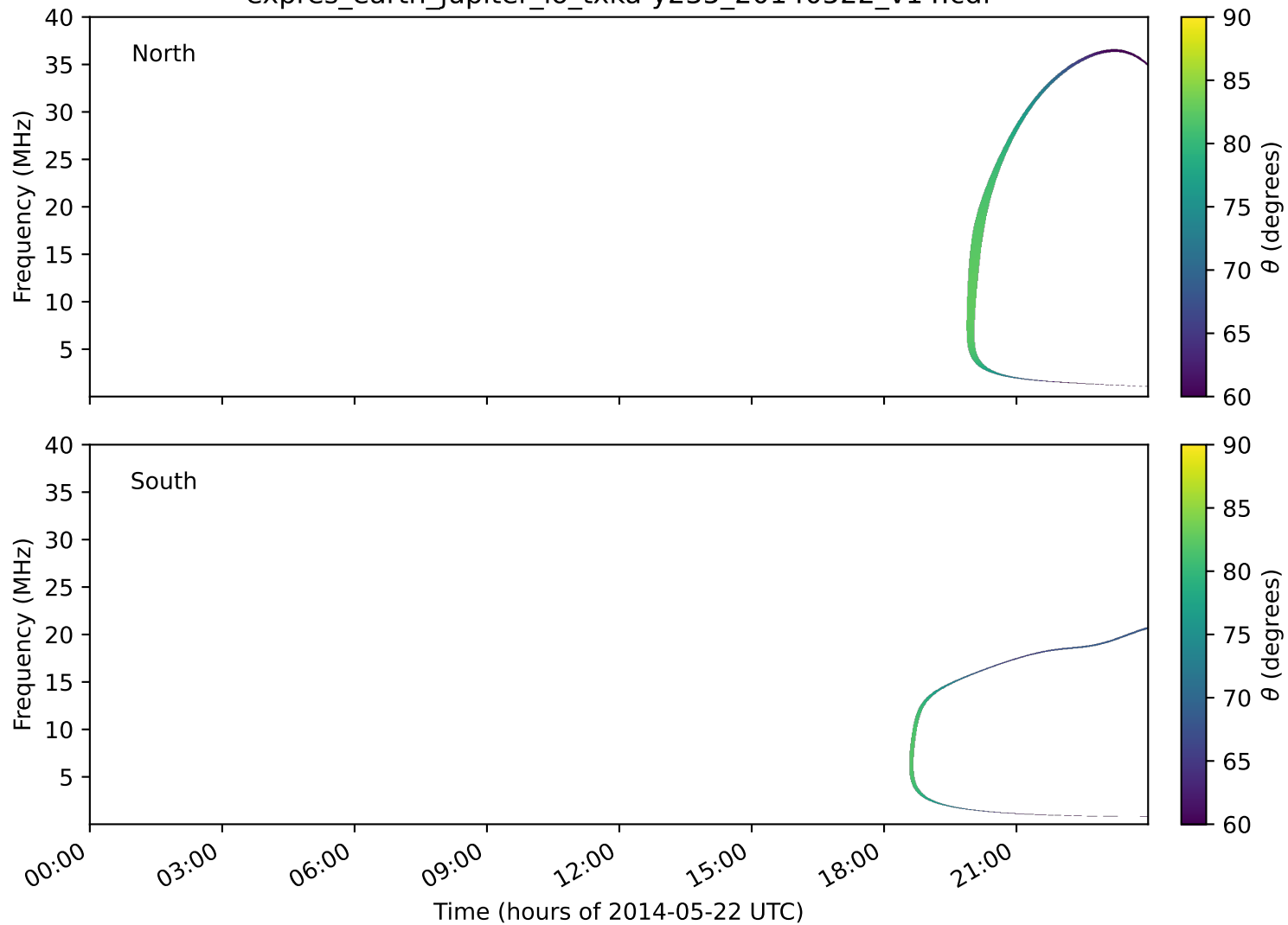
expres_earth_jupiter_io_txka-y235_20140522_v14.cdf
