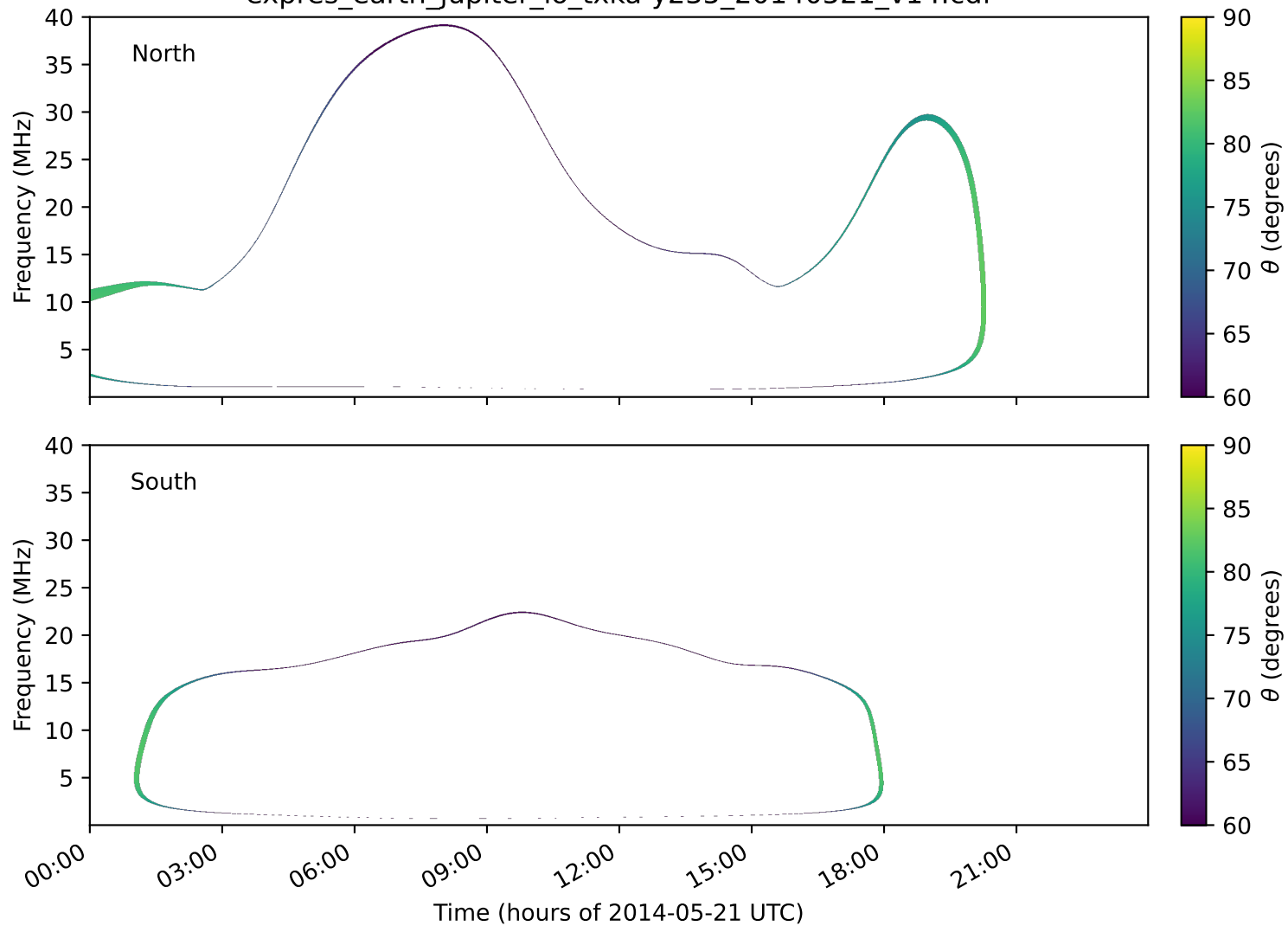
expres_earth_jupiter_io_txka-y235_20140521_v14.cdf
