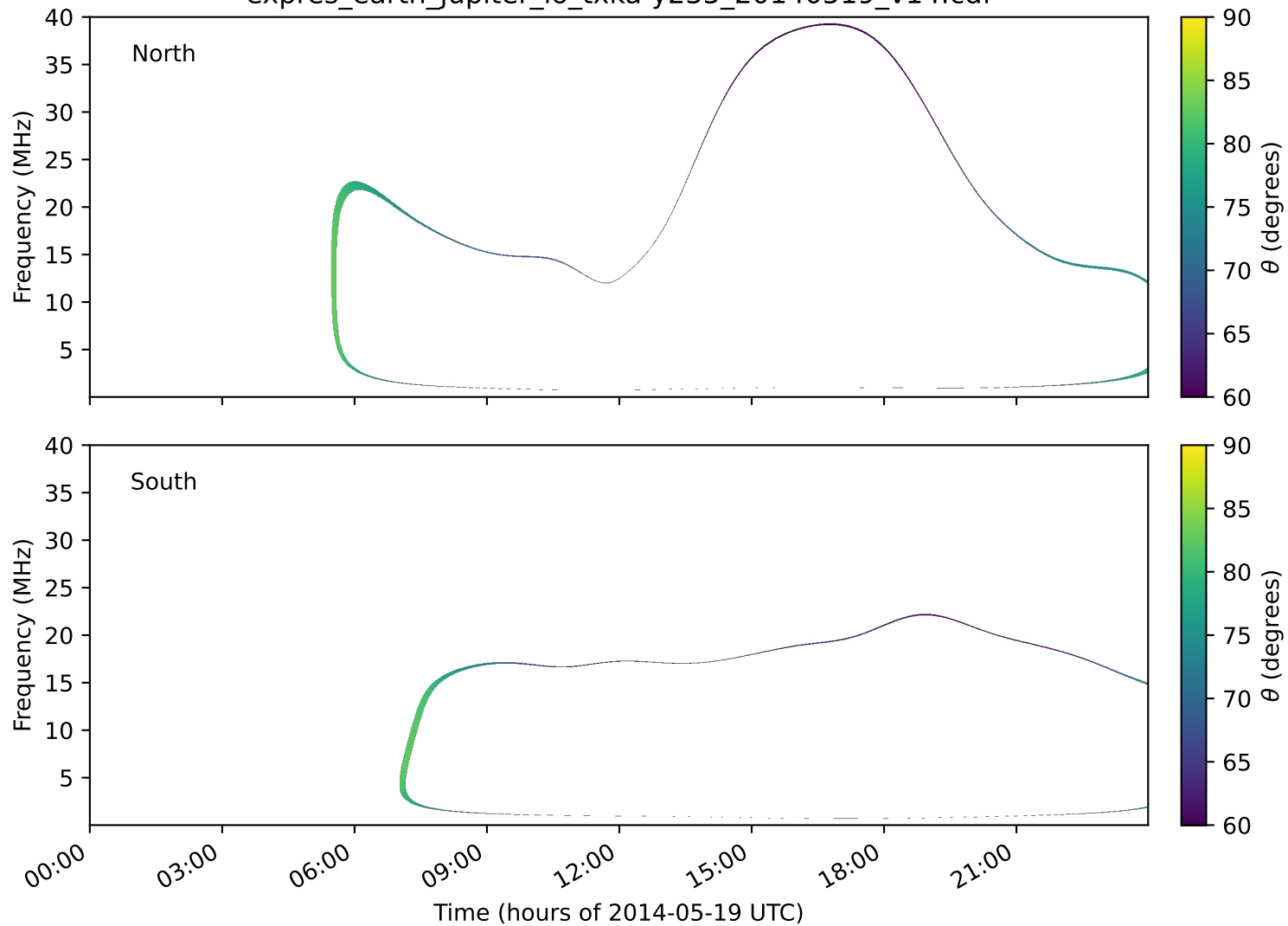
expres_earth_jupiter_io_txka-y235_20140519_v14.cdf
