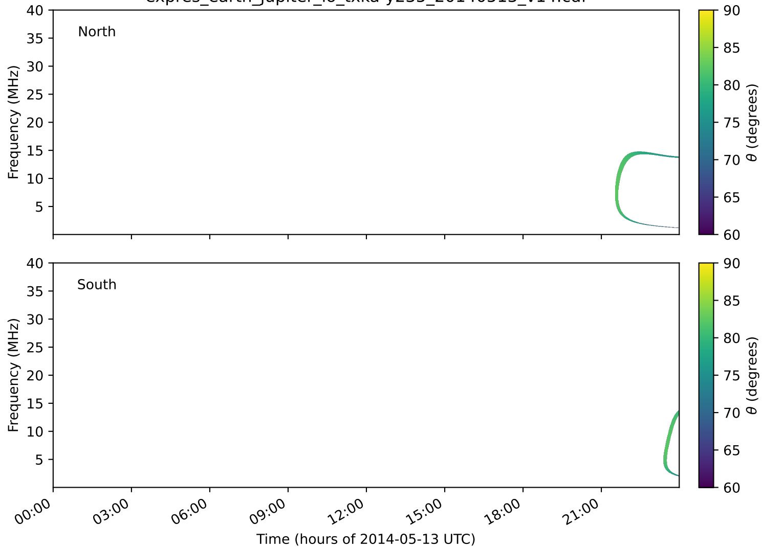
expres_earth_jupiter_io_txka-y235_20140513_v14.cdf
