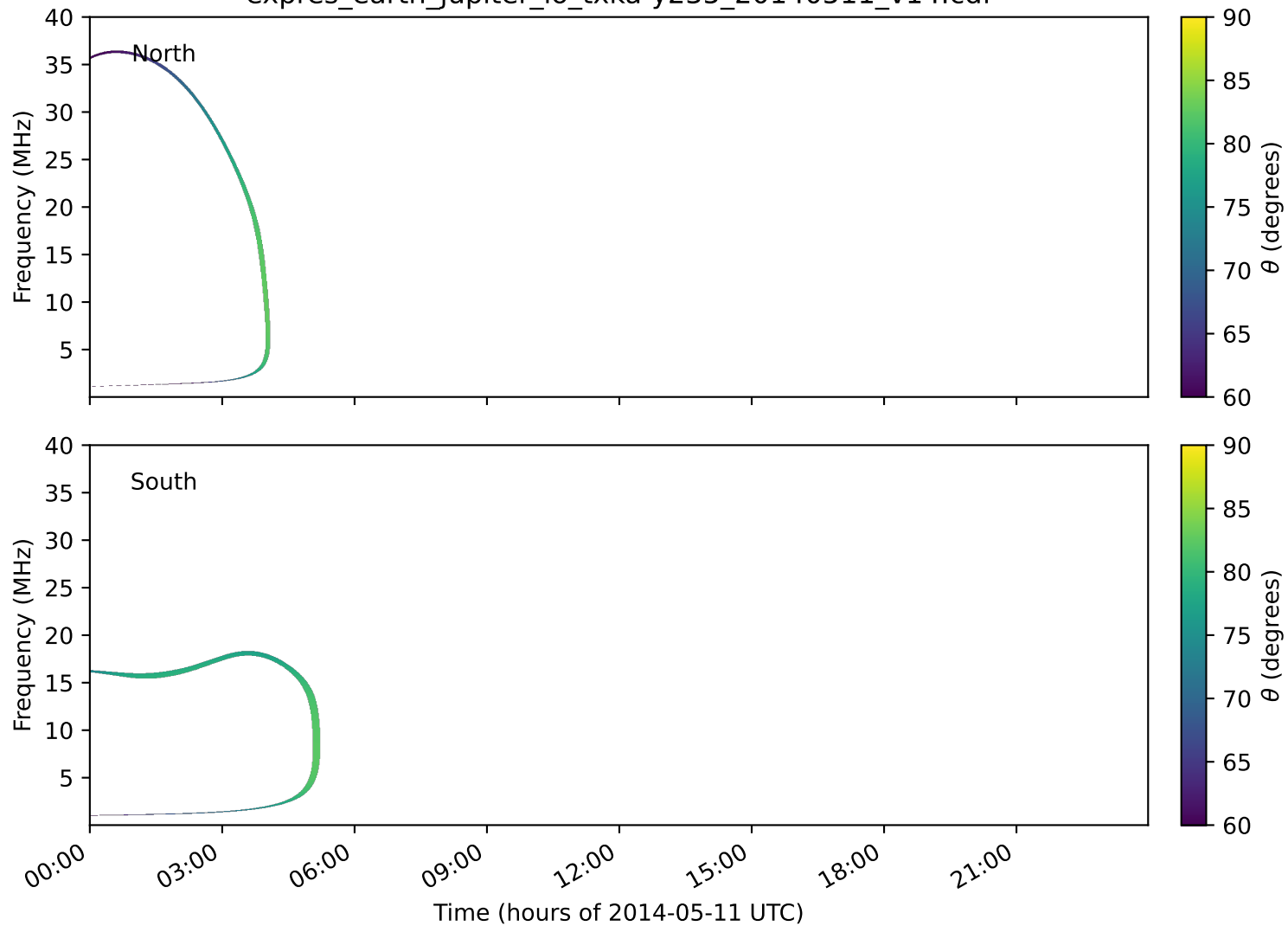
expres_earth_jupiter_io_txka-y235_20140511_v14.cdf
